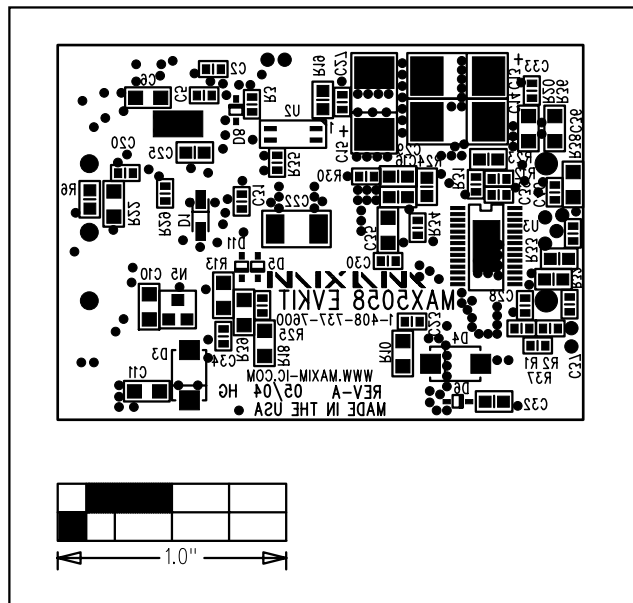
Figure 15. MAX5058 EV Kit Component Placement Guide—Solder Side
